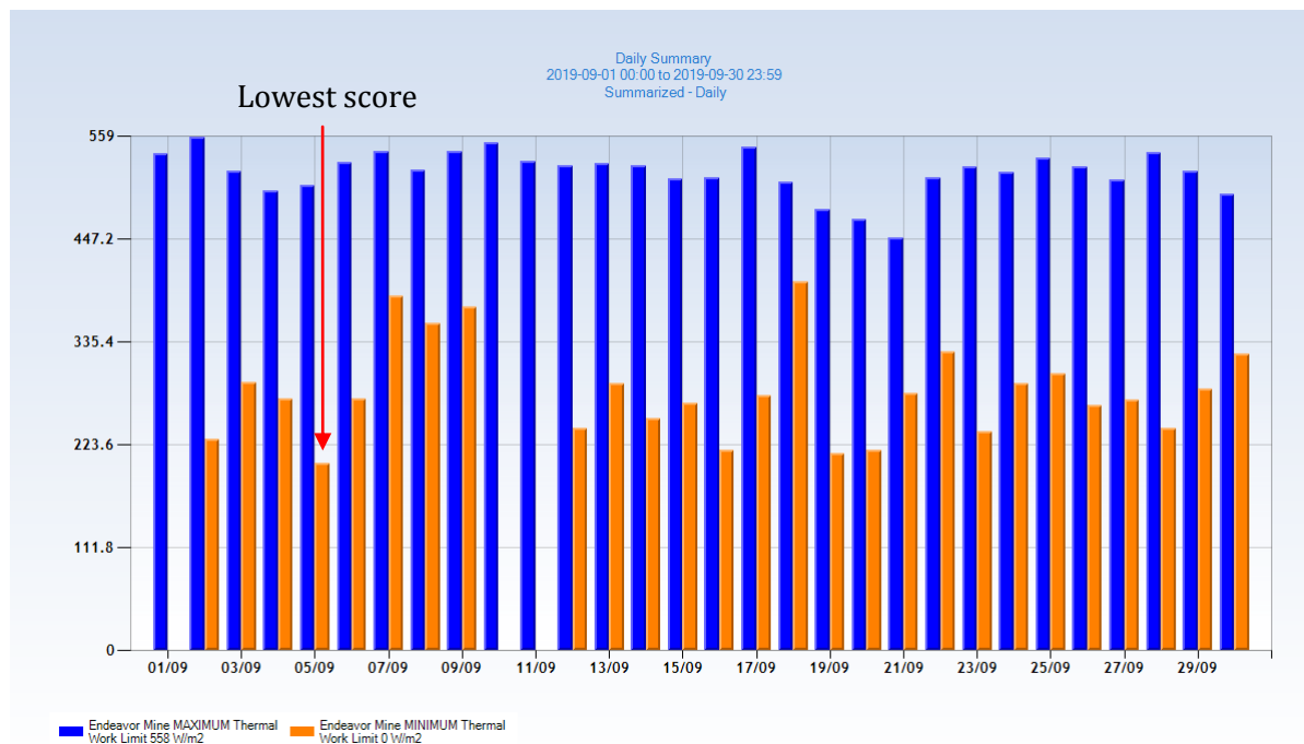
Figure 2.6 Thermal Work Limits: Maximum and Minimum Levels for September 2019
