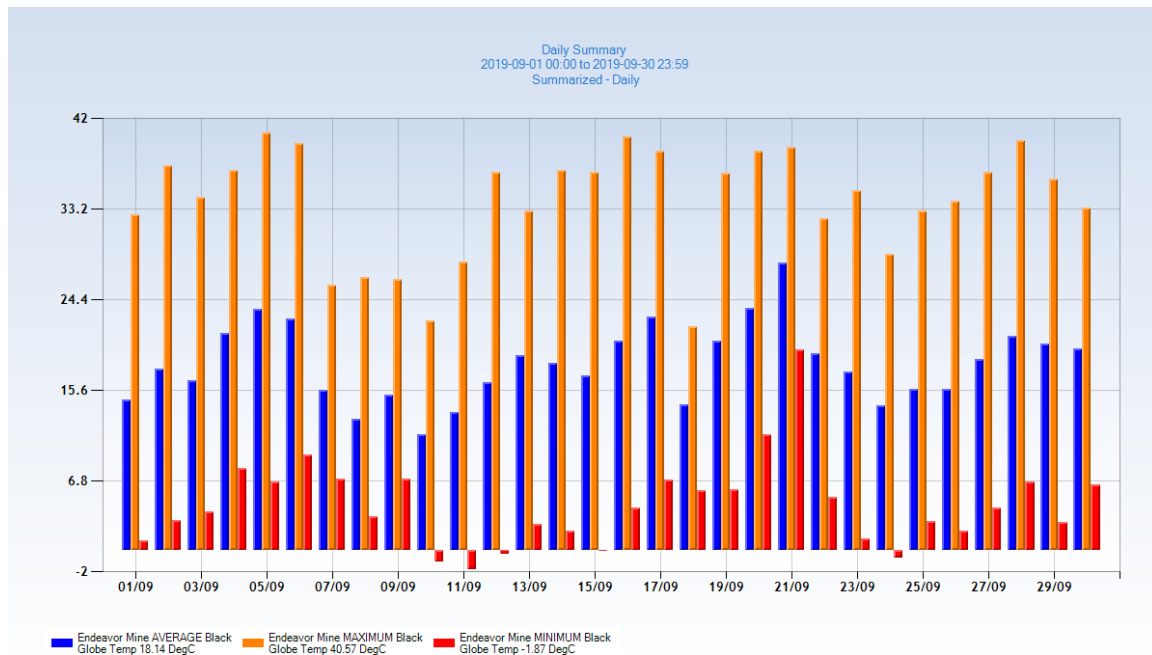
Figure 2.4 Min, Max and Ave Black Globe Temperature for September 2019
