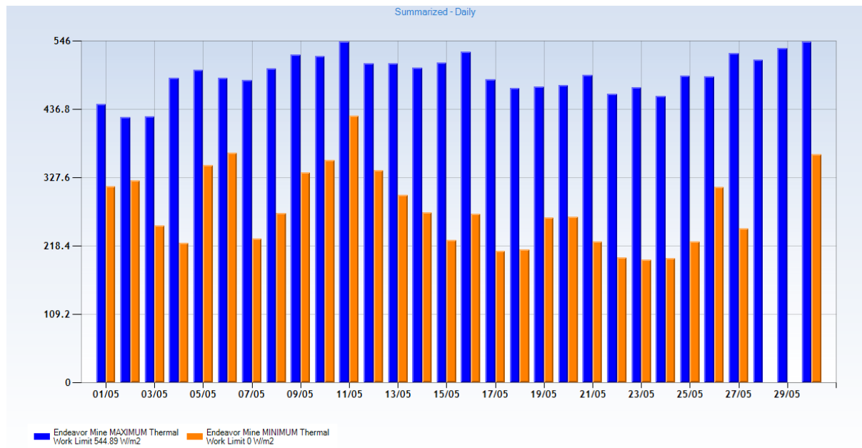
Figure 1.5: Thermal Work Limits: Maximum and Minimum Levels for May 2019
