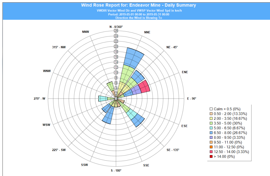
Figure 1.8: Wind Rose for the Endeavor Mine for May 2019
