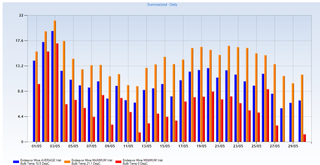
Figure 1.3: Daily Max, Min and Ave Wet Bulb Temperature Levels for May 2019
