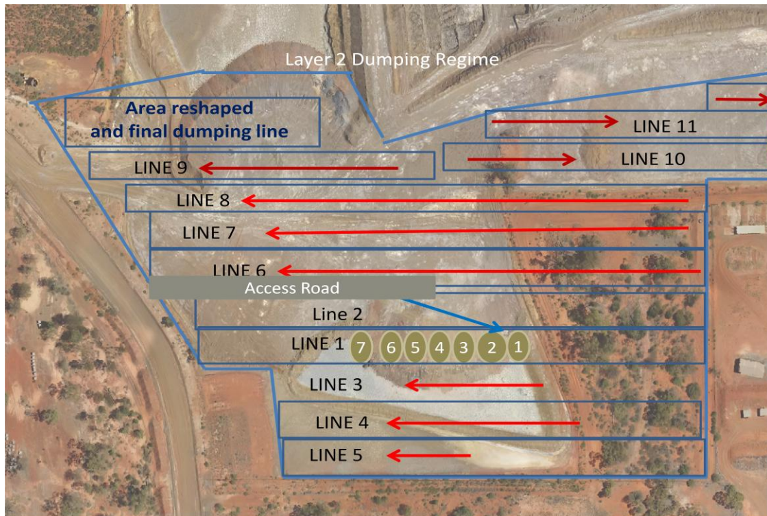
Figure 11.2: Waste rock placement plan
